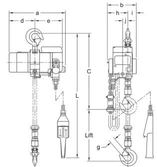
TCR500P Single Fall Pendant Model
